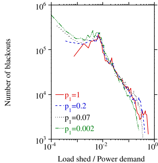
Figure 9. Frequency distribution of blackouts for different values of the probability for an overload line to outage.
