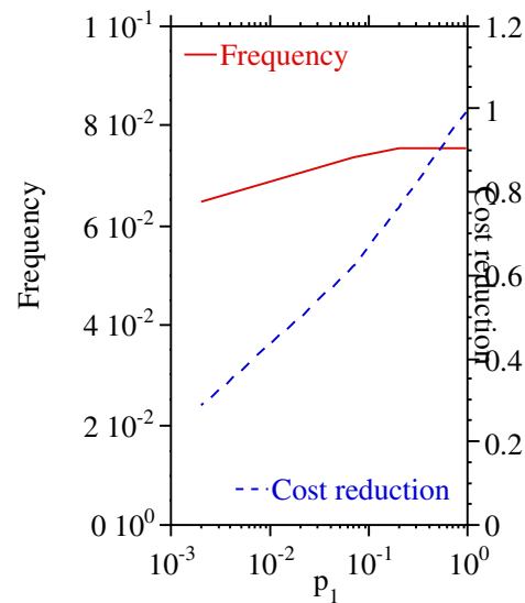
Figure 10. frequency of blackouts and their estimated cost as a function of the probability for an overload line to outage.
