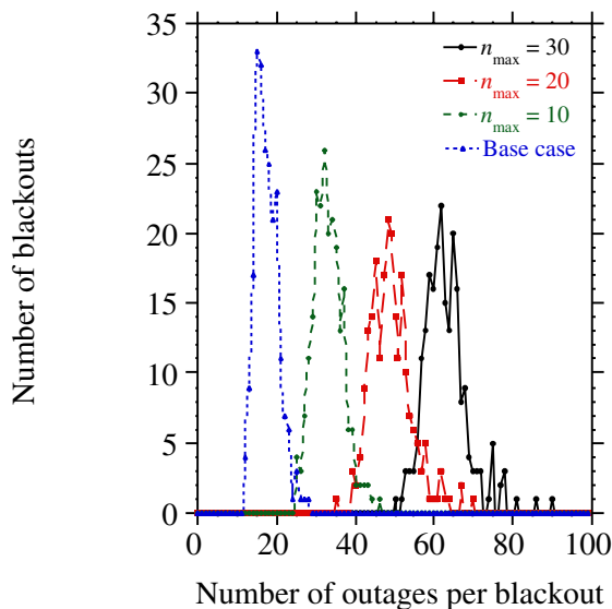
Figure 6. Distribution of the worst yearly blackouts for different level of mitigation.
