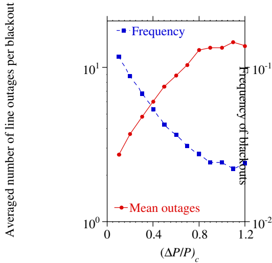
Figure 12. Frequency of blackouts and averaged number of outages per blackout as a function of (\Delta P/P)_c for a tree network with 46 nodes.
