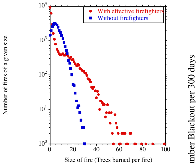
Figure 3. Frequency of forest fire sizes with and without fire fighting.
