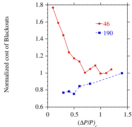
Figure 14. Normalized cost of the blackouts as a function of (\Delta P/P)_c for two different tree networks.
