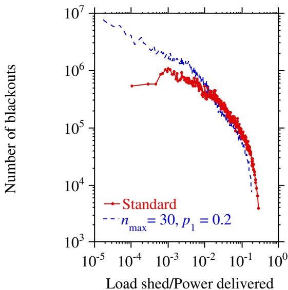
Figure 11. Distribution of the normalized load shed during blackouts for a case combining two mitigation methods and the same distribution for the base case.
