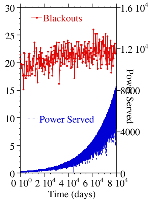
Figure 4. Time evolution of the power served and number of blackouts per year from the OPA model.
