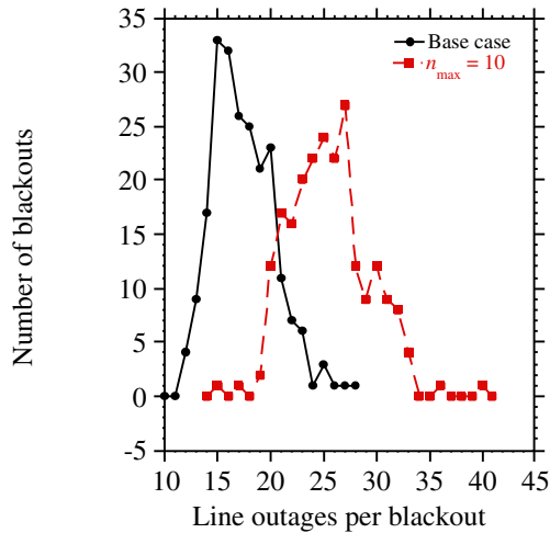
Figure 8. Distribution of the worst yearly blackouts for the base case and for n_{max} = 10 .
