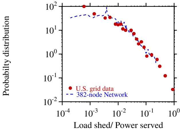
Figure 1. Blackout probability distribution vs. blackout size.
