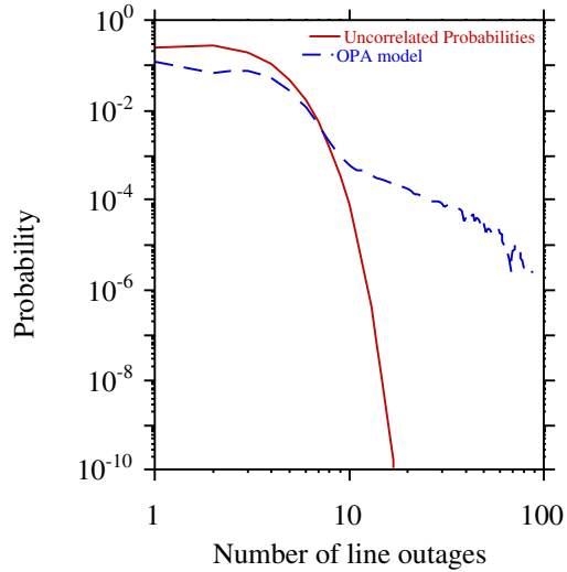
Figure 2. Blackout probability distribution vs. blackout size for uncorrelated probabilities and for the dynamical OPA model.
