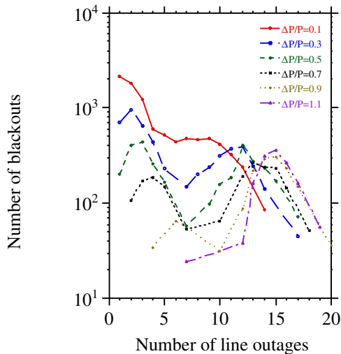
Figure 13. Frequency of blackouts as a function of number of line outages for different values of (\Delta P/P)_c .
