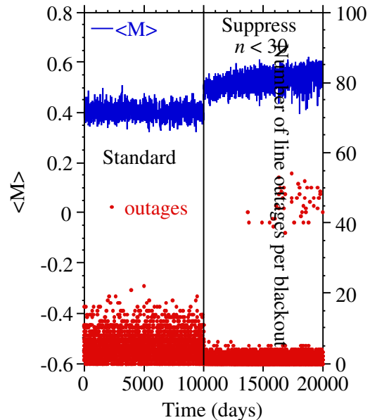
Figure 7. Time evolution of the number of outages per blackout and \langle M \rangle before and after the mitigation action has been applied.
