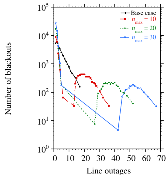
Figure 5. Logarithm of the number of blackouts as a function of the number of line outages for different values of n_{\max} .
